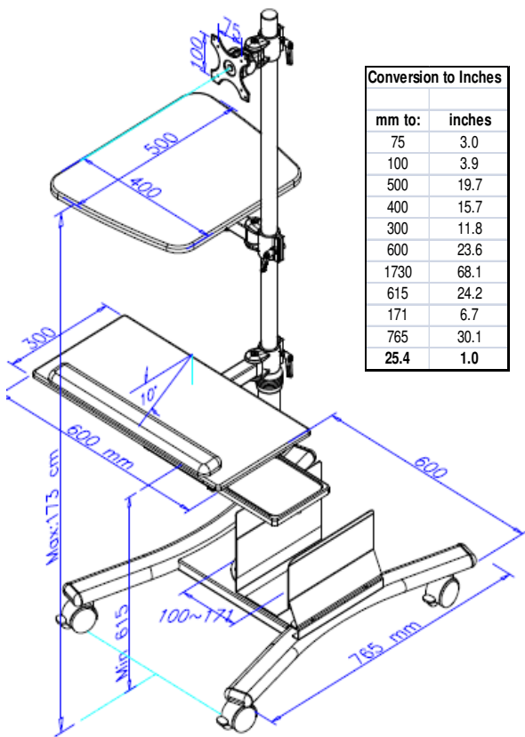
CUZZI VC03 Mobile LCD Pole Workstation
